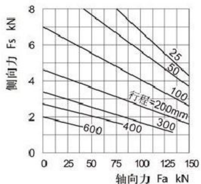
图7 SWL10/15(QWL10/15)
